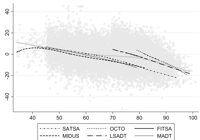
Fig. 2 Locally weighted regression curves of the standardized grip strength on age for all women in the total sample as well as in the single studies. The thick gray curve is for the total sample
