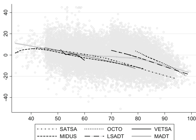
Fig. 1 Locally weighted regression curves of the standardized grip strength on age for all men in the total sample as well as in the single studies. The thick gray curve is for the total sample
